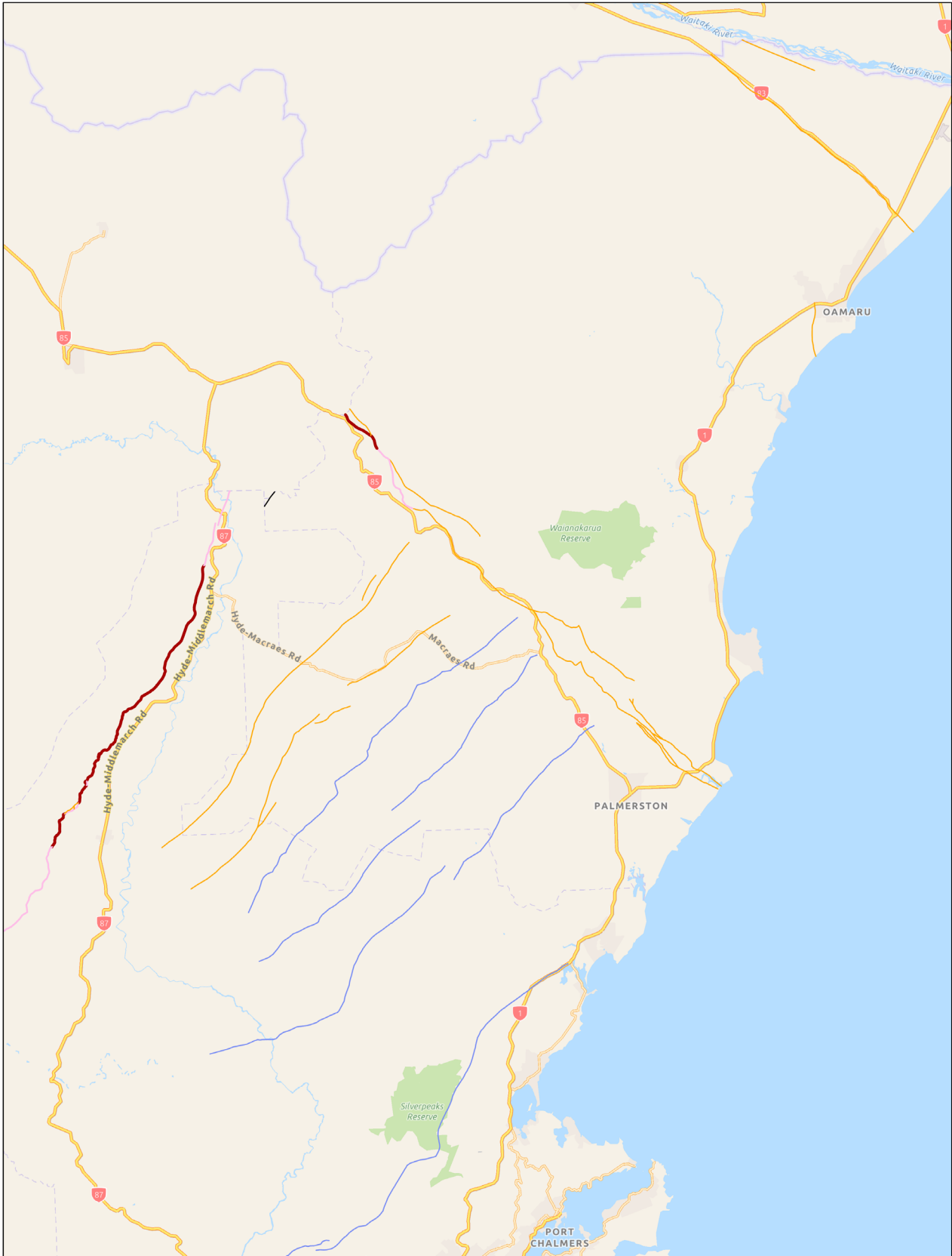
Fault Lines - Waiheмо
